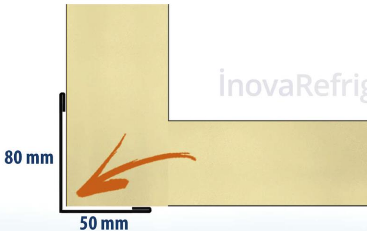
80 mm*50 mm External Corner Mounting Profile L Metal Sheet
