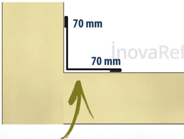
70 mm*70 mm Inner Corner Mounting Profile L Metal Sheet
