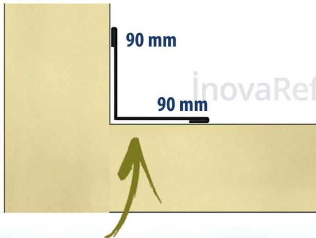
90 mm*90 mm Inner Corner Mounting Profile L Metal Sheet
