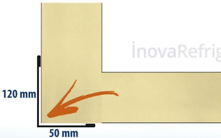
120 mm*50 mm External Corner Mounting Profile L Metal Sheet
