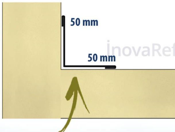
50 mm*50 mm Inner Corner Mounting Profile L Metal Sheet
